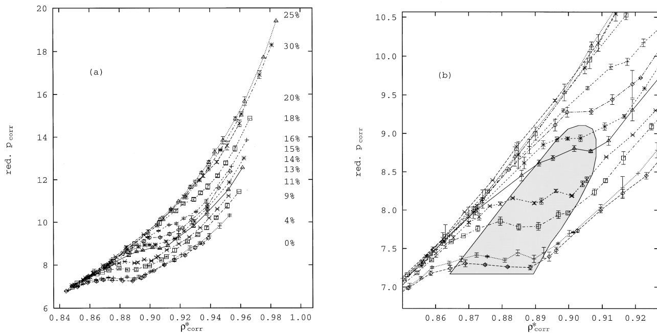
FIG. 5. (a) State diagram: reduced pressure versus density, both hard-core corrected for different bidispersities ( \delta r_b = 0\% - 30\% , system L45). (b) Zoom of the plateau region in the state diagram of (a); the gray area points as a guide to the eye to the coexisting region.
